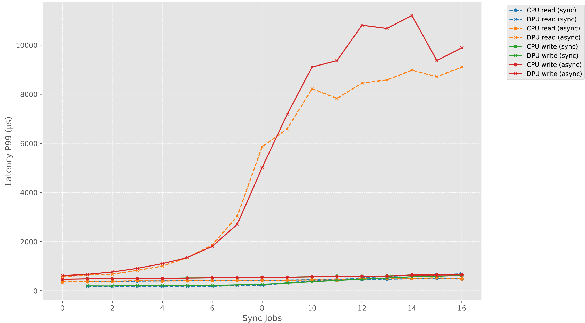
Latency P99 vs Sync Jobs (async1 syncN) - SEQ (CPU vs DPU)
